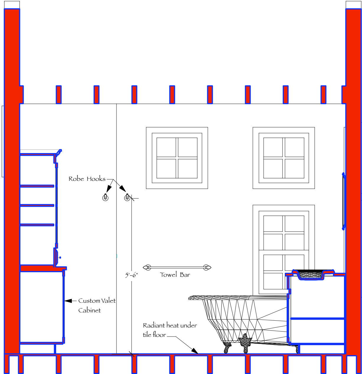
NORTH ELEVATION
