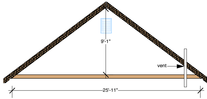
Attic Section
